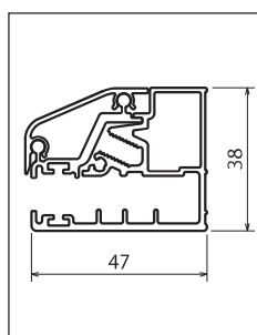
Standard profile side panel KP01GA1FI-K
